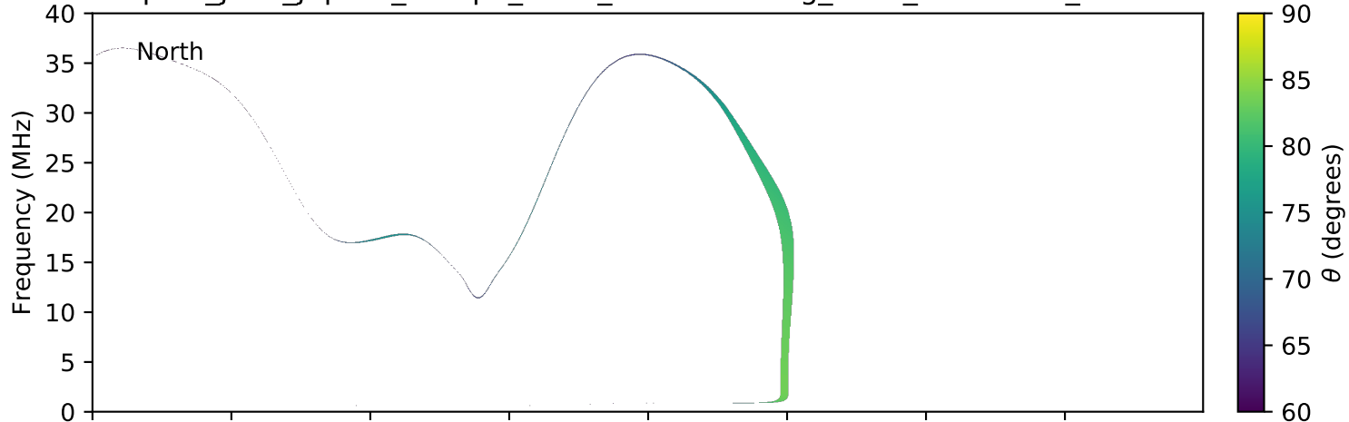
expres_juno_jupiter_europa_isaac_lossc-wid1deg_3kev_20160208_v01.cdf
