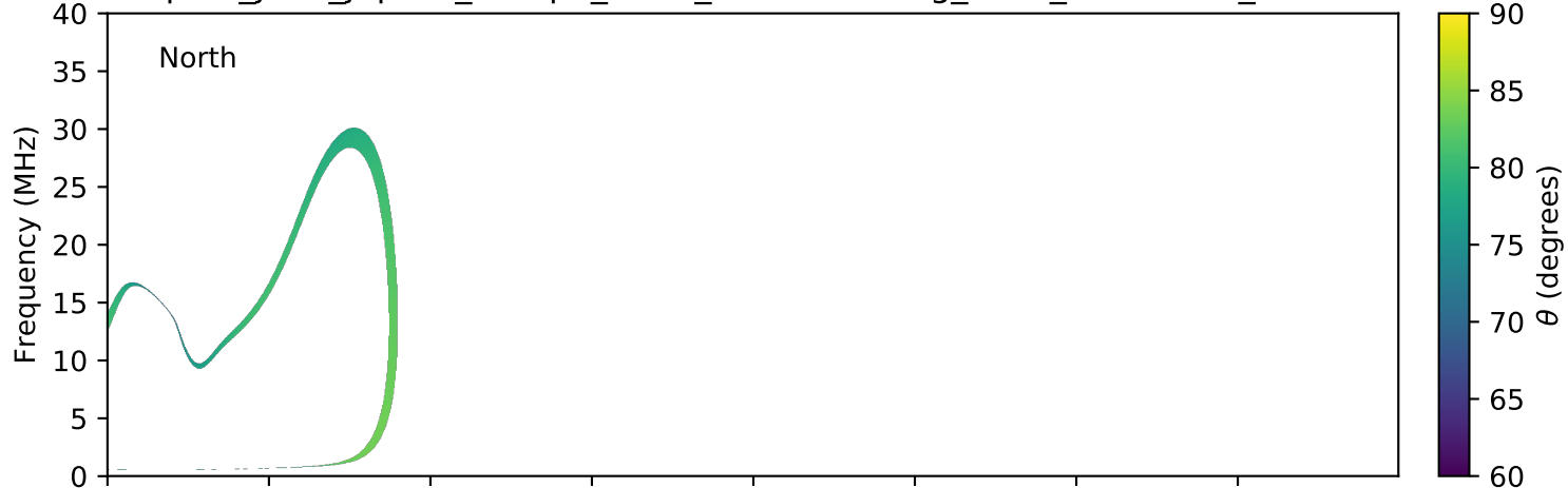
expres_juno_jupiter_europa_isaac_lossc-wid1deg_3kev_20160205_v01.cdf
