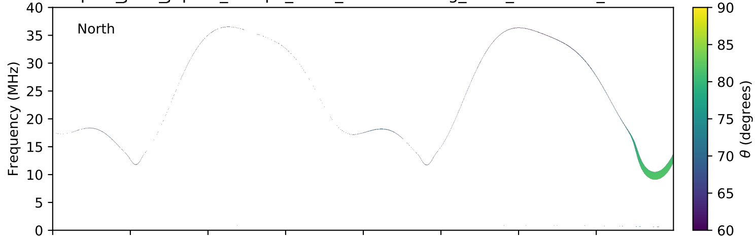
expres_juno_jupiter_europa_isaac_lossc-wid1deg_3kev_20160204_v01.cdf
