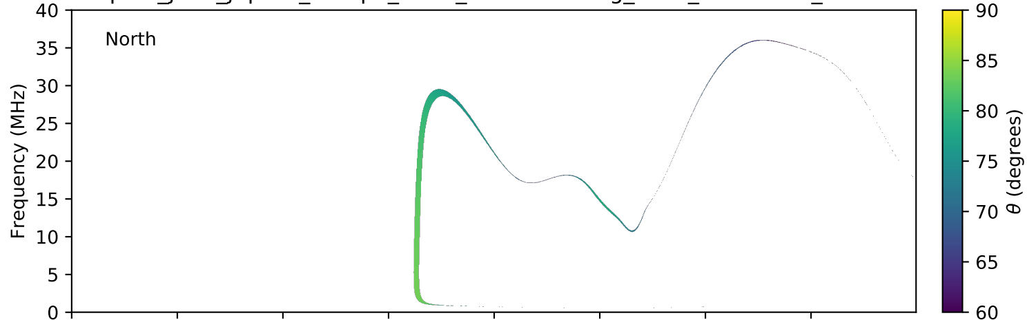
expres_juno_jupiter_europa_isaac_lossc-wid1deg_3kev_20160203_v01.cdf
