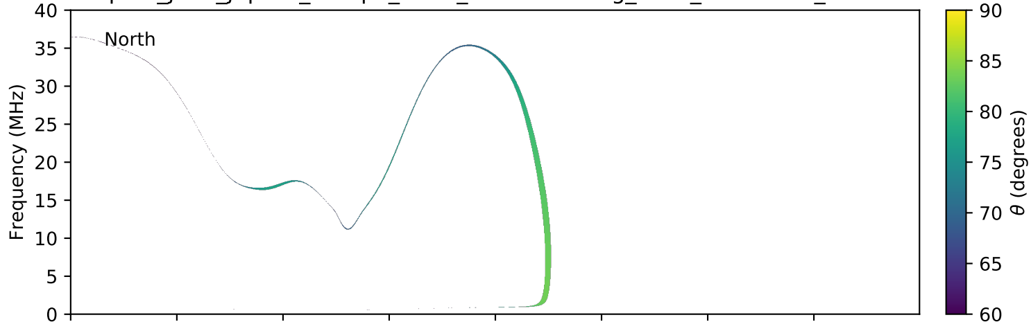
expres_juno_jupiter_europa_isaac_lossc-wid1deg_3kev_20160201_v01.cdf
