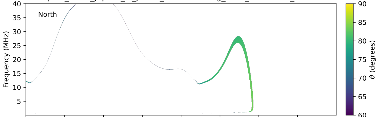
expres_earth_jupiter_io_jrm33_lossc-wid1deg_3kev_20191225_v11.cdf
