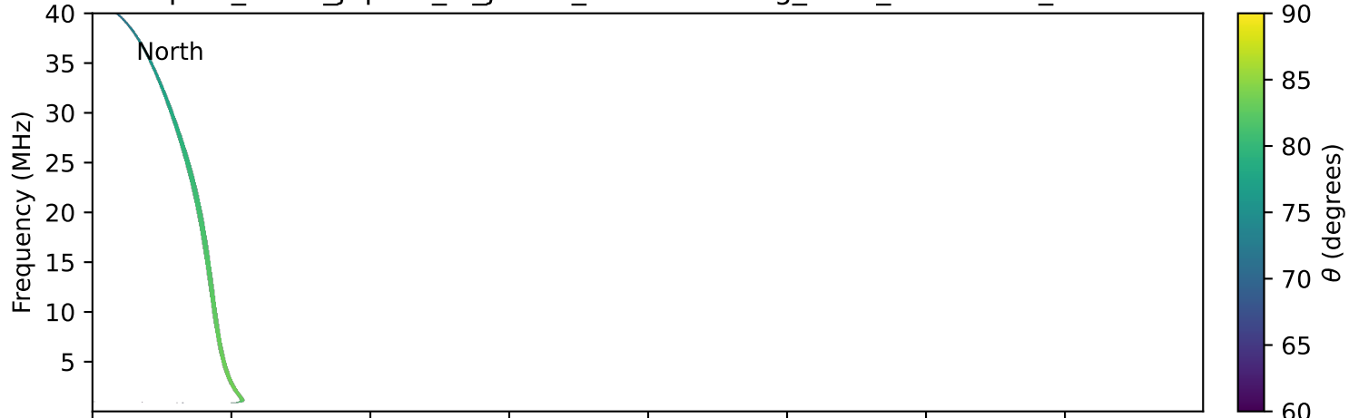
expres_earth_jupiter_io_jrm33_lossc-wid1deg_3kev_20191222_v11.cdf
