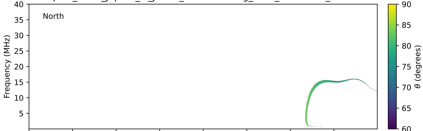
expres_earth_jupiter_io_jrm33_lossc-wid1deg_3kev_20191217_v11.cdf
