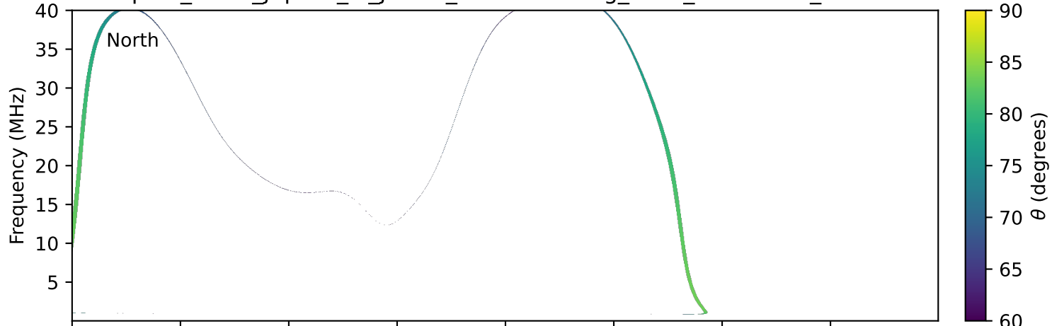
expres_earth_jupiter_io_jrm33_lossc-wid1deg_3kev_20191209_v11.cdf
