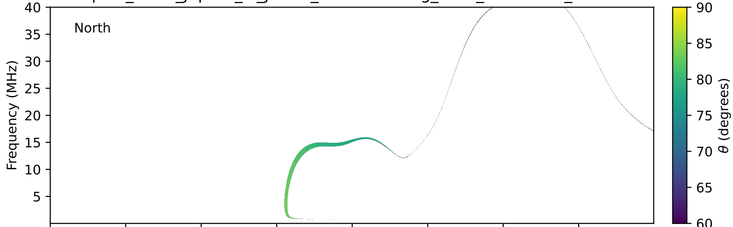
expres_earth_jupiter_io_jrm33_lossc-wid1deg_3kev_20191205_v11.cdf
