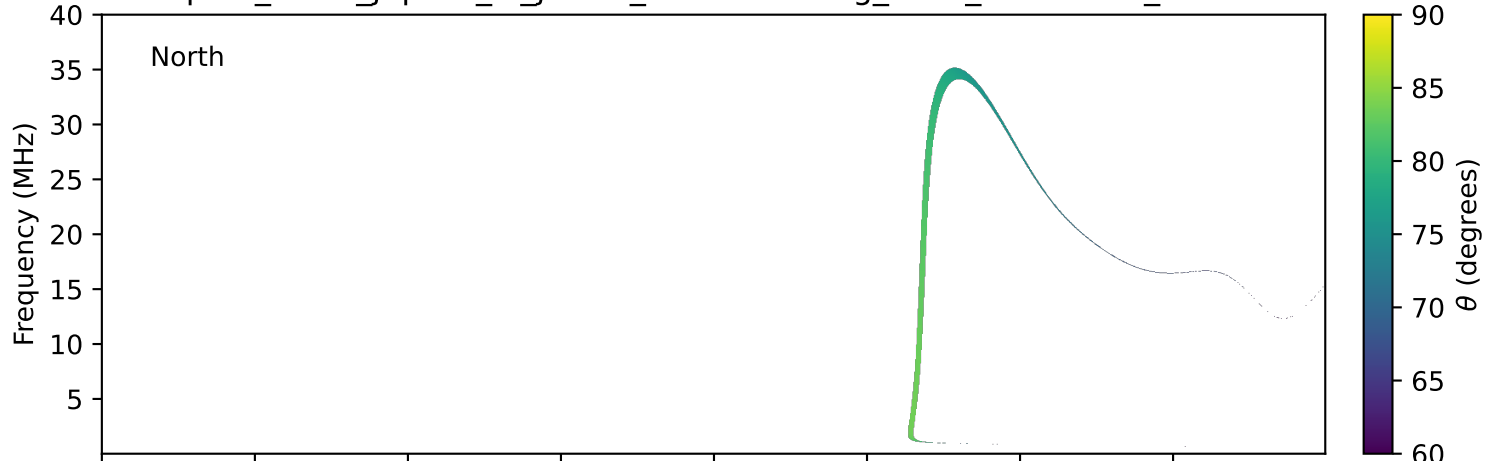
expres_earth_jupiter_io_jrm33_lossc-wid1deg_3kev_20191203_v11.cdf
