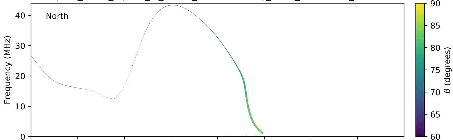
expres_earth_jupiter_io_jrm09_lossc-wid1deg_3kev_20191229_v01.cdf
