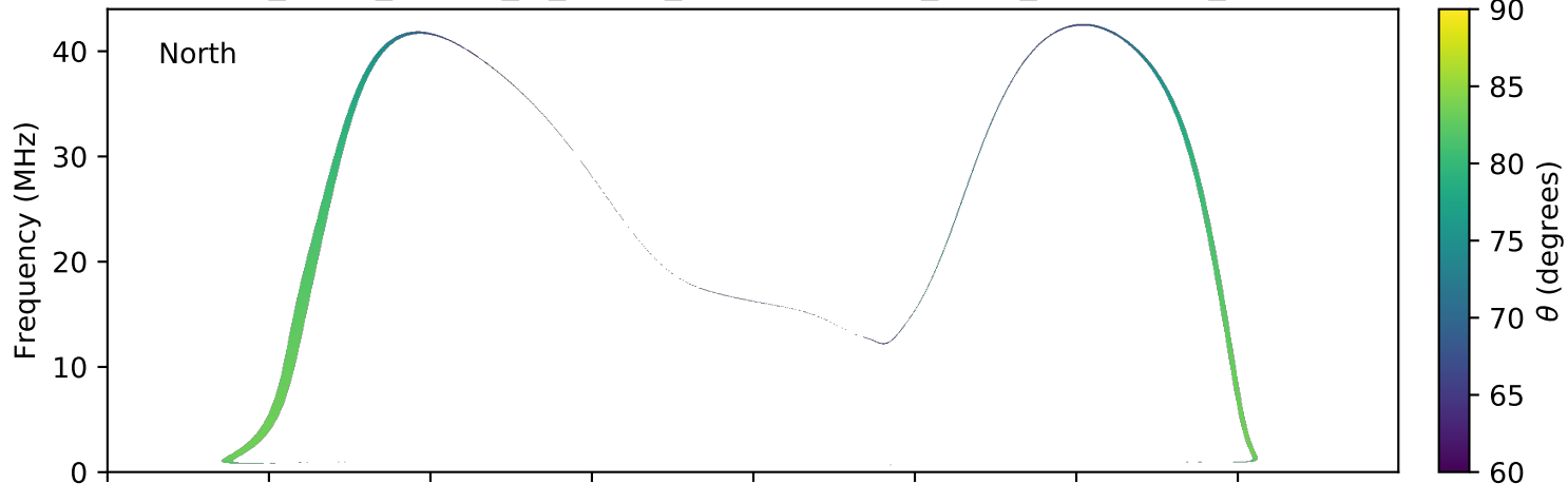
expres_earth_jupiter_io_jrm09_lossc-wid1deg_3kev_20191227_v01.cdf
