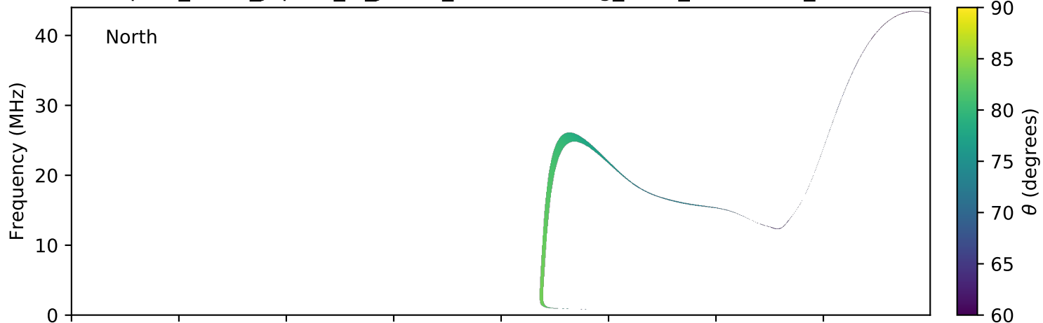
expres_earth_jupiter_io_jrm09_lossc-wid1deg_3kev_20191223_v01.cdf
