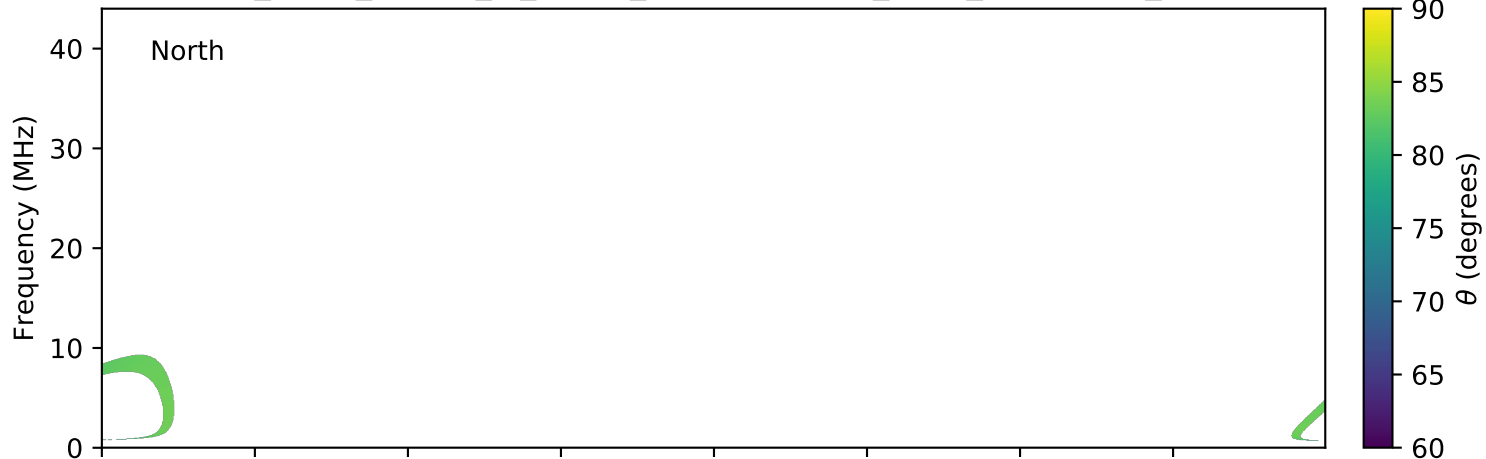
expres_earth_jupiter_io_jrm09_lossc-wid1deg_3kev_20191219_v01.cdf
