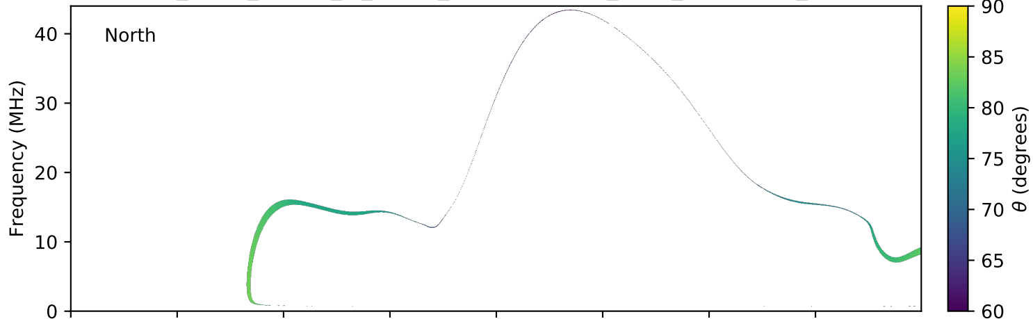
expres_earth_jupiter_io_jrm09_lossc-wid1deg_3kev_20191218_v01.cdf
