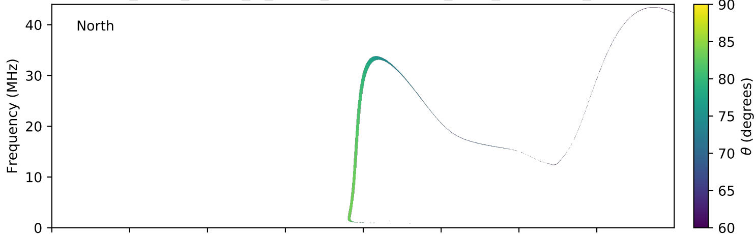
expres_earth_jupiter_io_jrm09_lossc-wid1deg_3kev_20191216_v01.cdf
