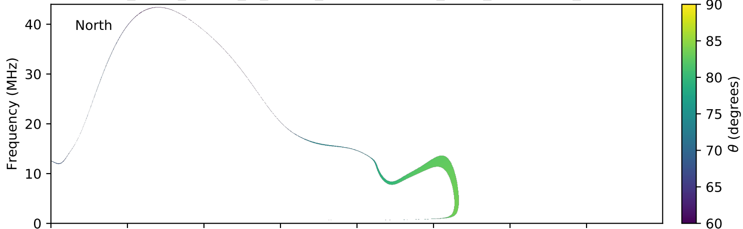
expres_earth_jupiter_io_jrm09_lossc-wid1deg_3kev_20191206_v01.cdf
