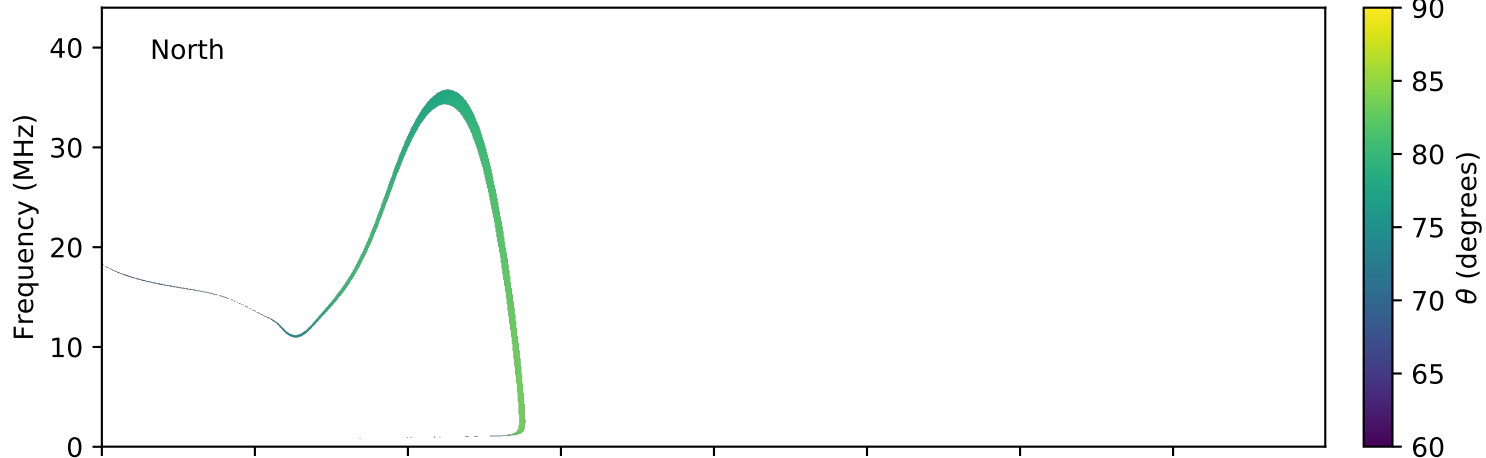
expres_earth_jupiter_io_jrm09_lossc-wid1deg_3kev_20191201_v01.cdf
