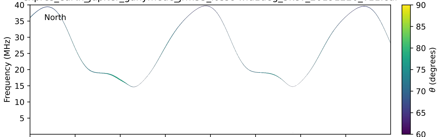
expres_earth_jupiter_ganymede_jrm33_lossc-wid1deg_3kev_20191226_v11.cdf
