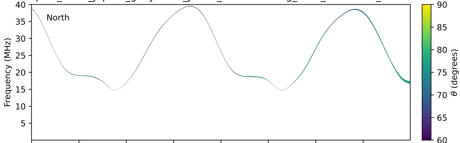
expres_earth_jupiter_ganymede_jrm33_lossc-wid1deg_3kev_20191205_v11.cdf
