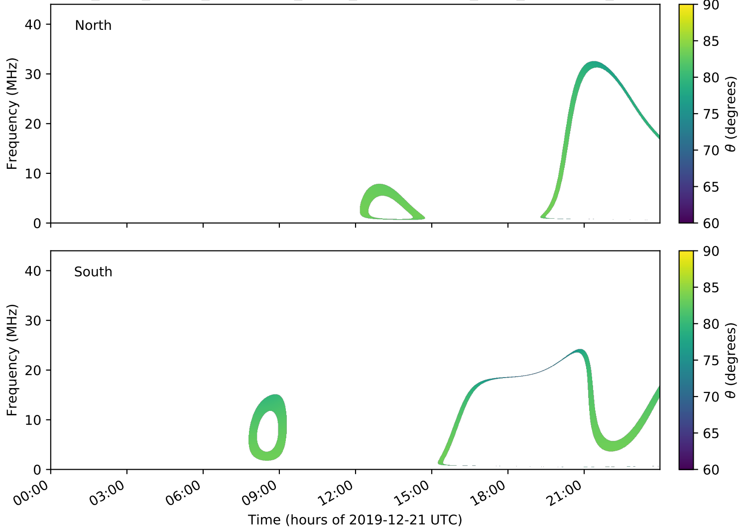
expres_earth_jupiter_ganymede_jrm09_lossc-wid1deg_3kev_20191221_v01.cdf
