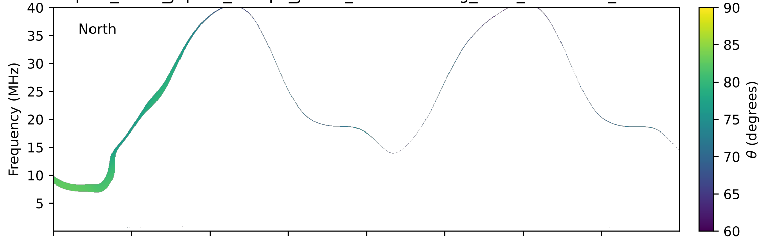
expres_earth_jupiter_europa_jrm33_lossc-wid1deg_3kev_20191215_v11.cdf
