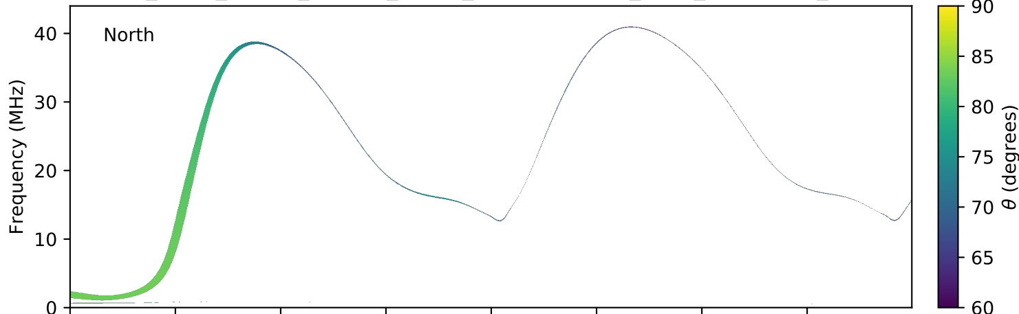
expres_earth_jupiter_europa_jrm09_lossc-wid1deg_3kev_20191220_v01.cdf
