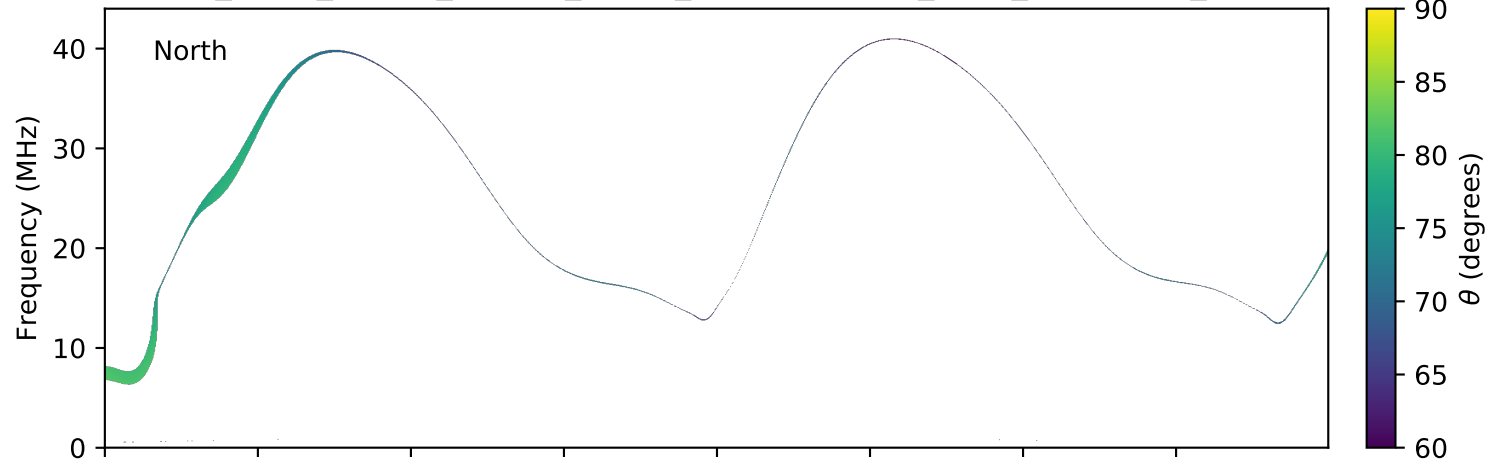
expres_earth_jupiter_europa_jrm09_lossc-wid1deg_3kev_20191213_v01.cdf
