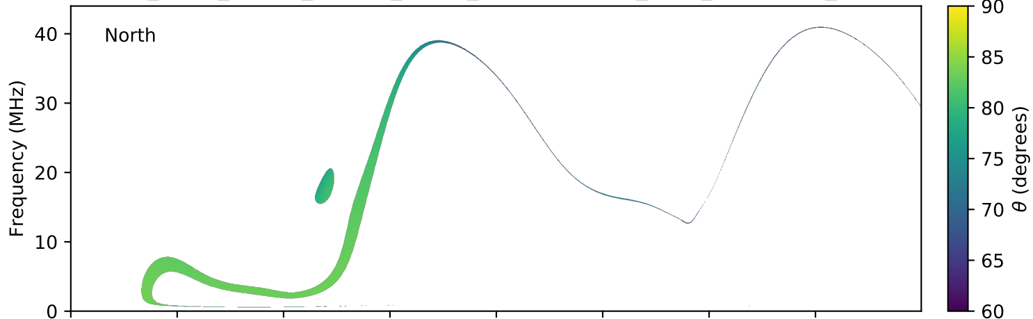
expres_earth_jupiter_europa_jrm09_lossc-wid1deg_3kev_20191202_v01.cdf
