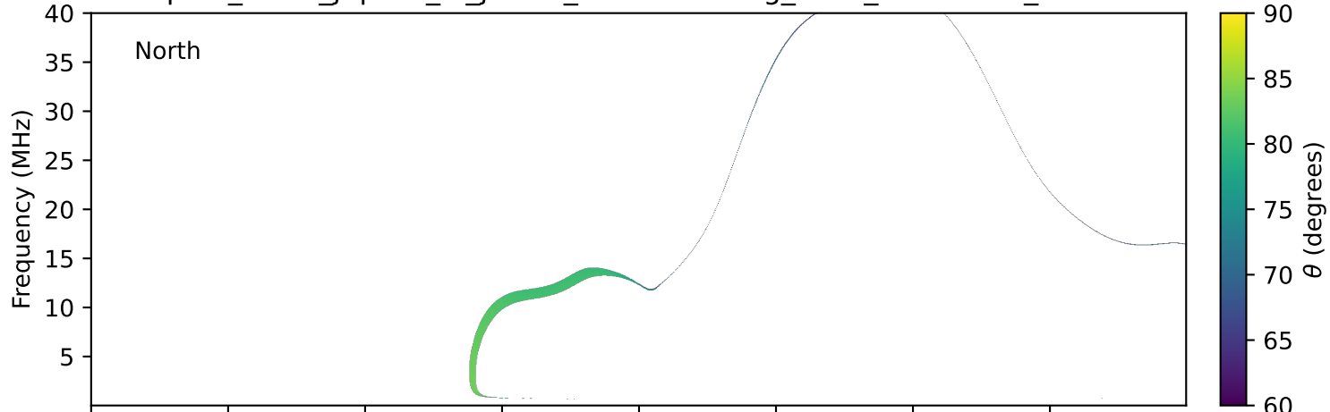
expres_earth_jupiter_io_jrm33_lossc-wid1deg_3kev_20191121_v11.cdf
