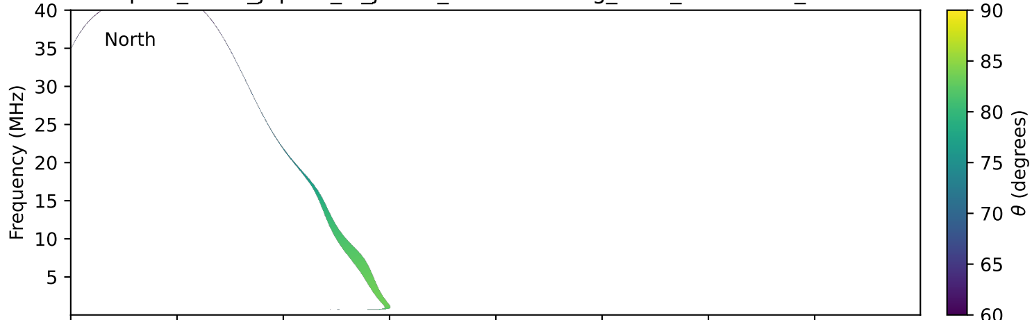
expres_earth_jupiter_io_jrm33_lossc-wid1deg_3kev_20191120_v11.cdf
