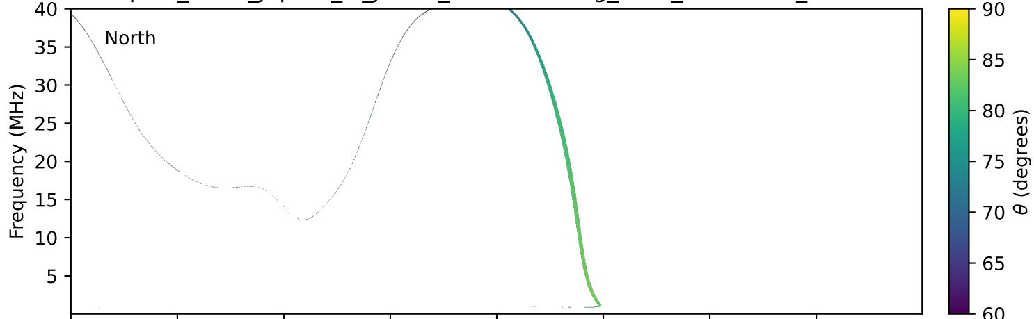
expres_earth_jupiter_io_jrm33_lossc-wid1deg_3kev_20191118_v11.cdf
