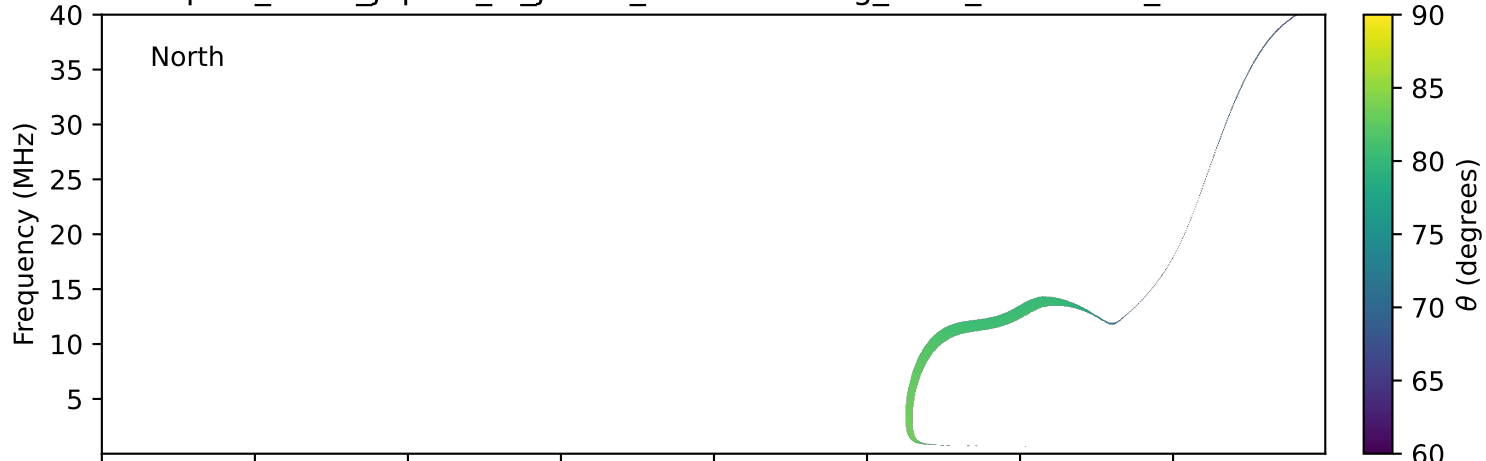
expres_earth_jupiter_io_jrm33_lossc-wid1deg_3kev_20191112_v11.cdf
