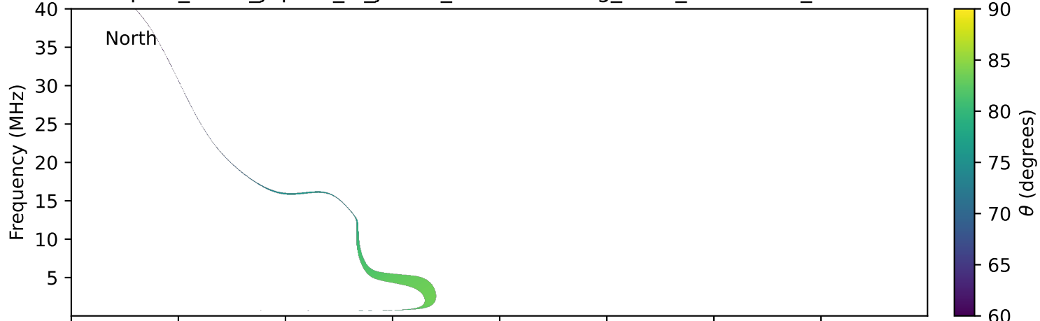
expres_earth_jupiter_io_jrm33_lossc-wid1deg_3kev_20191106_v11.cdf
