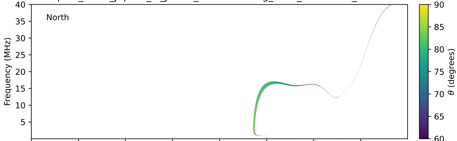
expres_earth_jupiter_io_jrm33_lossc-wid1deg_3kev_20191105_v11.cdf
