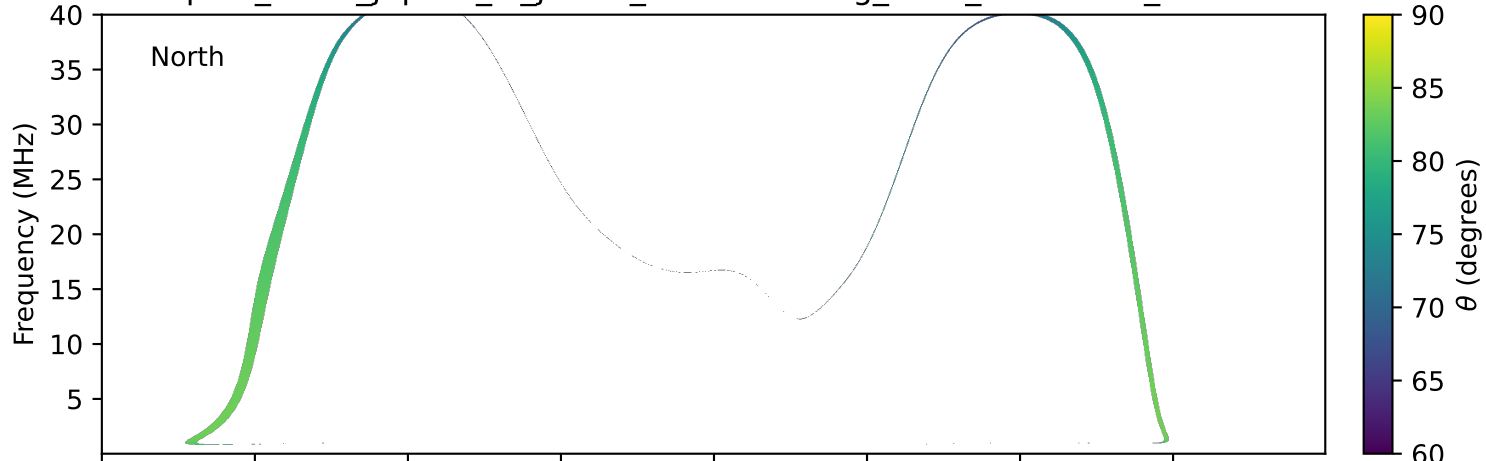
expres_earth_jupiter_io_jrm33_lossc-wid1deg_3kev_20191102_v11.cdf
