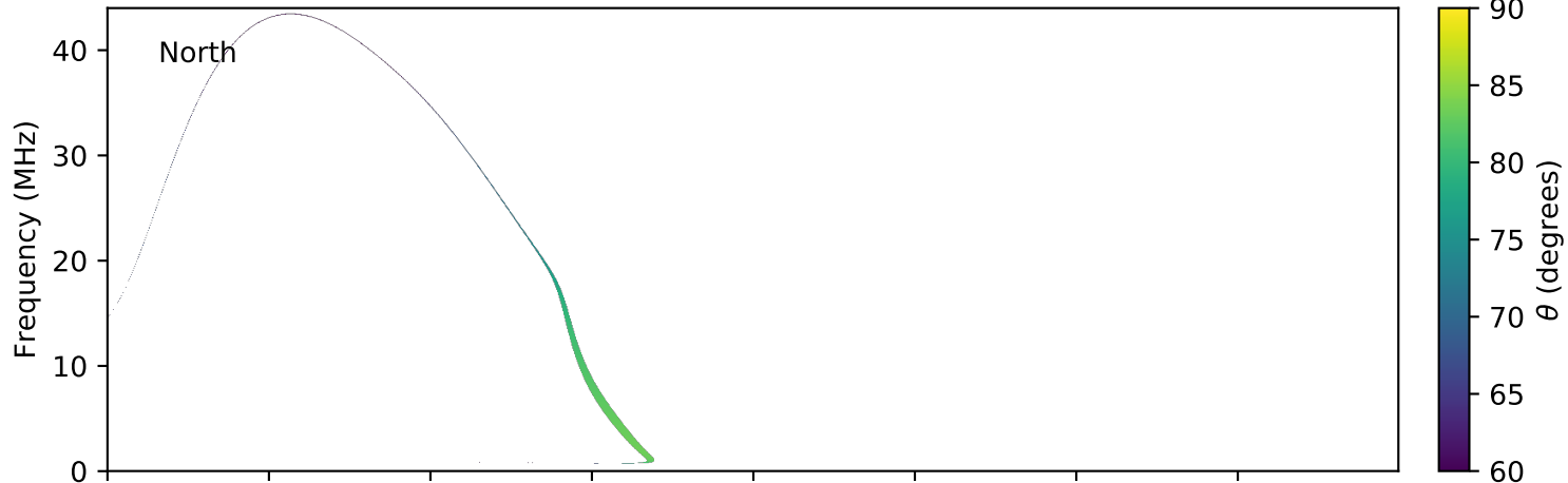
expres_earth_jupiter_io_jrm09_lossc-wid1deg_3kev_20191122_v01.cdf
