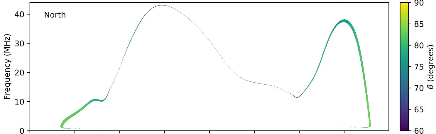
expres_earth_jupiter_io_jrm09_lossc-wid1deg_3kev_20191118_v01.cdf
