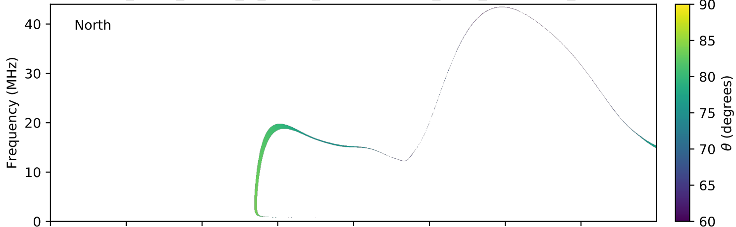
expres_earth_jupiter_io_jrm09_lossc-wid1deg_3kev_20191116_v01.cdf
