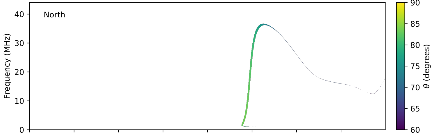
expres_earth_jupiter_io_jrm09_lossc-wid1deg_3kev_20191114_v01.cdf
