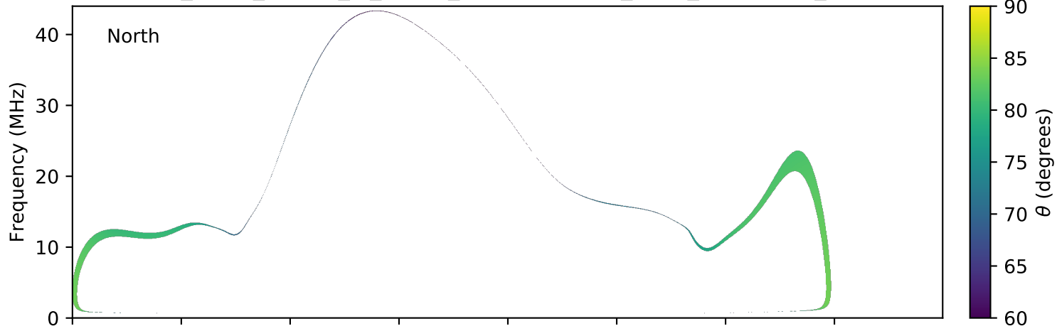
expres_earth_jupiter_io_jrm09_lossc-wid1deg_3kev_20191111_v01.cdf
