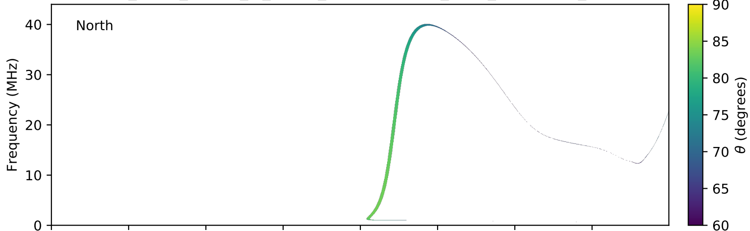
expres_earth_jupiter_io_jrm09_lossc-wid1deg_3kev_20191107_v01.cdf
