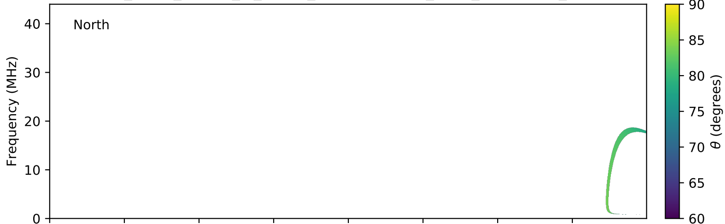
expres_earth_jupiter_io_jrm09_lossc-wid1deg_3kev_20191103_v01.cdf
