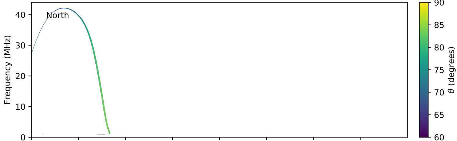
expres_earth_jupiter_io_jrm09_lossc-wid1deg_3kev_20191101_v01.cdf
