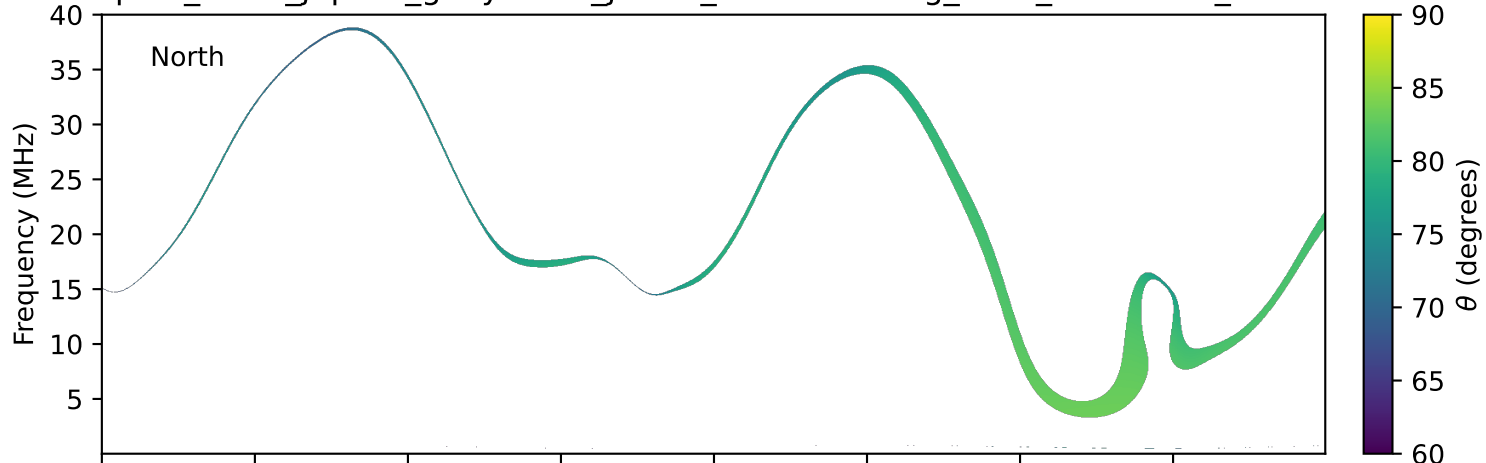
expres_earth_jupiter_ganymede_jrm33_lossc-wid1deg_3kev_20191110_v11.cdf
