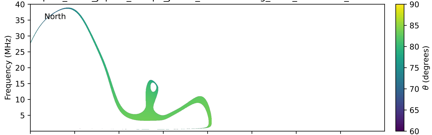
expres_earth_jupiter_europa_jrm33_lossc-wid1deg_3kev_20191125_v11.cdf
