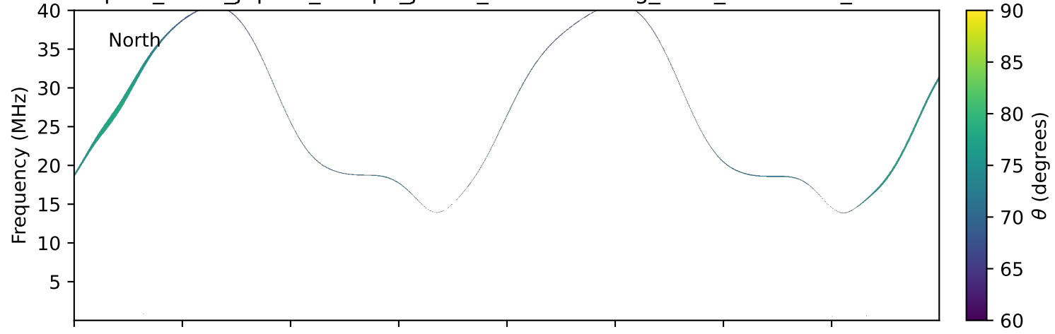
expres_earth_jupiter_europa_jrm33_lossc-wid1deg_3kev_20191117_v11.cdf
