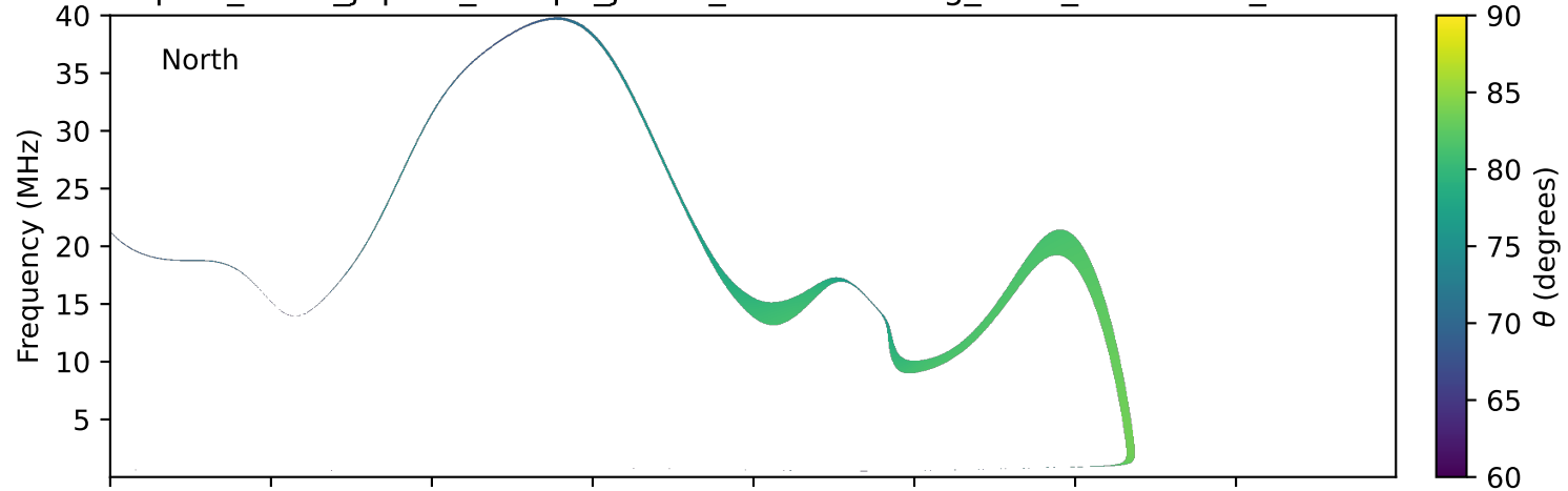
expres_earth_jupiter_europa_jrm33_lossc-wid1deg_3kev_20191114_v11.cdf
