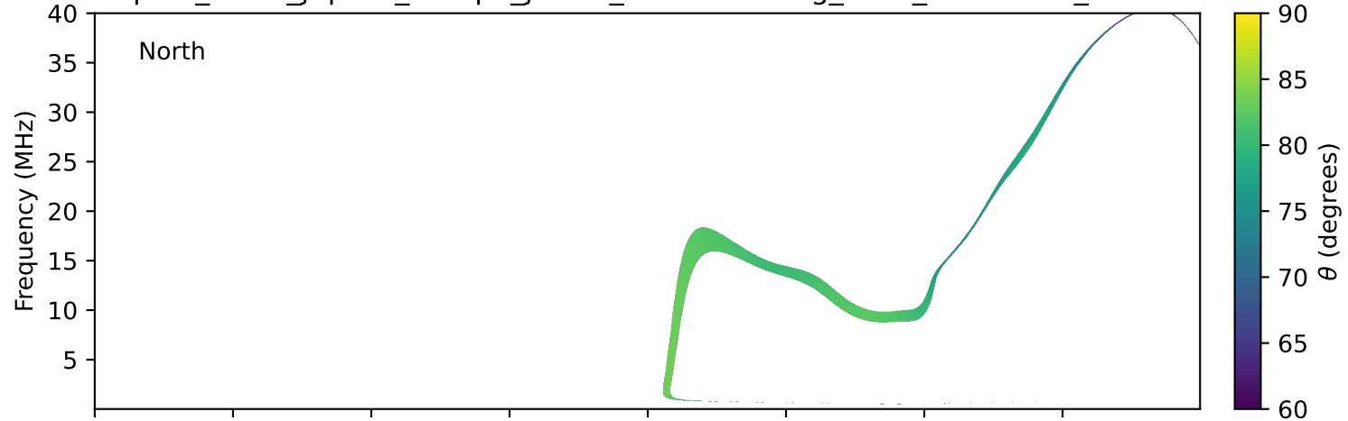
expres_earth_jupiter_europa_jrm33_lossc-wid1deg_3kev_20191110_v11.cdf
