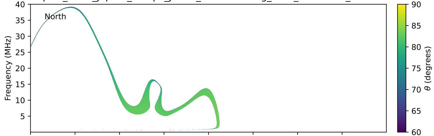
expres_earth_jupiter_europa_jrm33_lossc-wid1deg_3kev_20191101_v11.cdf
