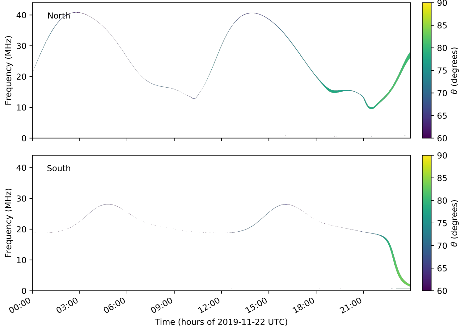
expres_earth_jupiter_europa_jrm09_lossc-wid1deg_3kev_20191122_v01.cdf
