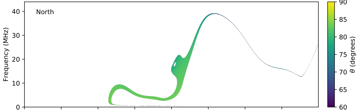
expres_earth_jupiter_europa_jrm09_lossc-wid1deg_3kev_20191114_v01.cdf
