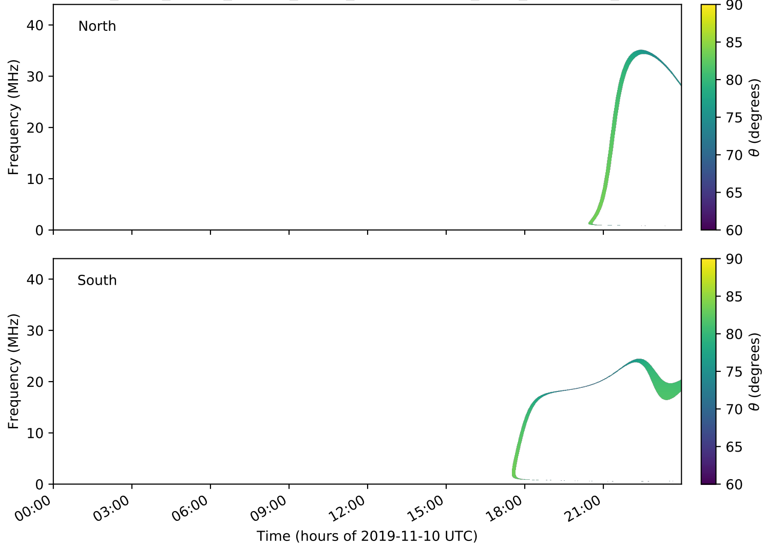
expres_earth_jupiter_europa_jrm09_lossc-wid1deg_3kev_20191110_v01.cdf
